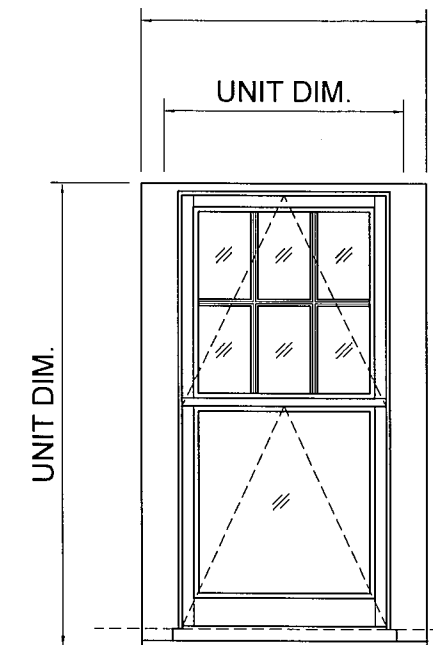
EXTERIOR ELEVATION OF SERIES 5000 DOUBLE HUNG FOLD-UP IN WINDOW UNIT AT COUNTER
